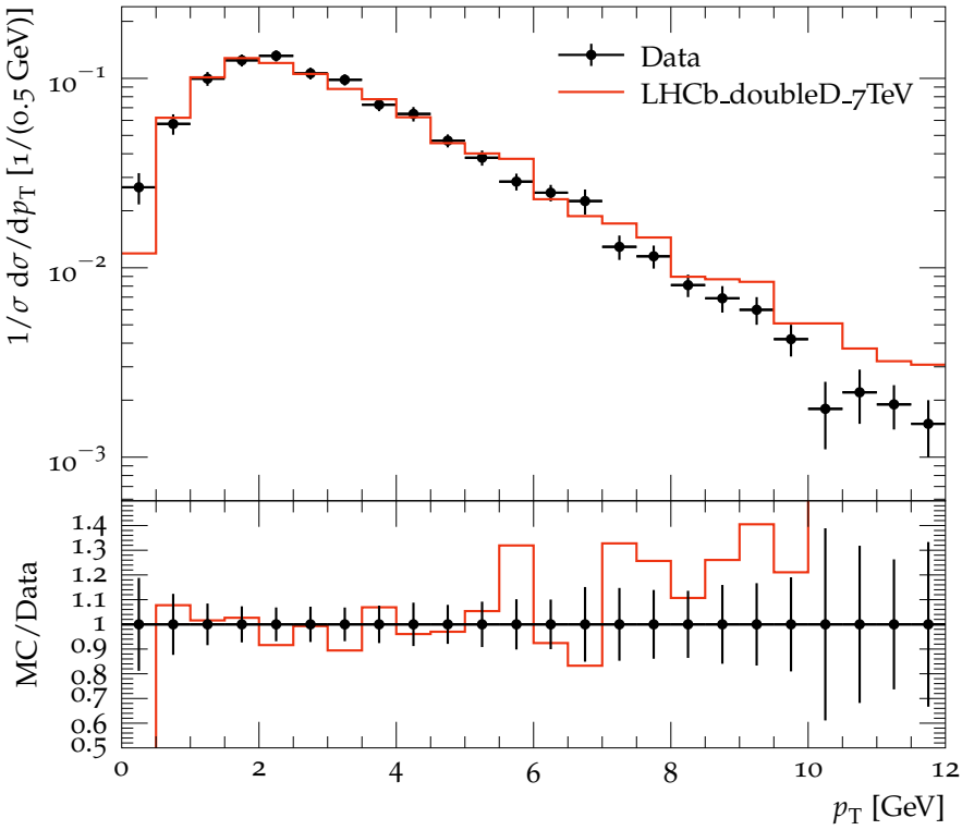
p_T distribution of J/\Psi for J/\Psi D^0 pairs
