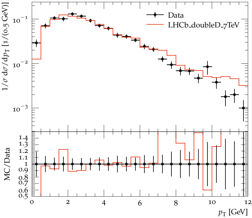
p_T distribution of J/\Psi for J/\Psi D^+ pairs
