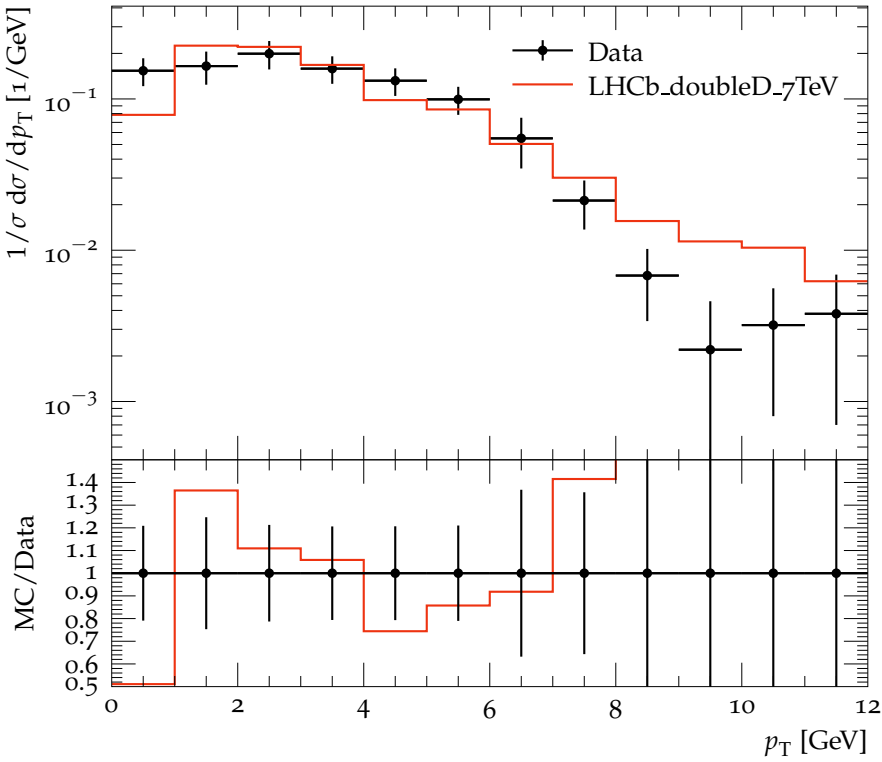
p_T distribution of J/\Psi for J/\Psi D_s^+ pairs
