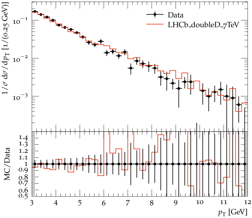
p_T distribution of D^0 for J/\Psi D^0 pairs
