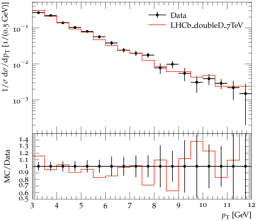
p_T distribution of D^+ for J/\Psi D^+ pairs
