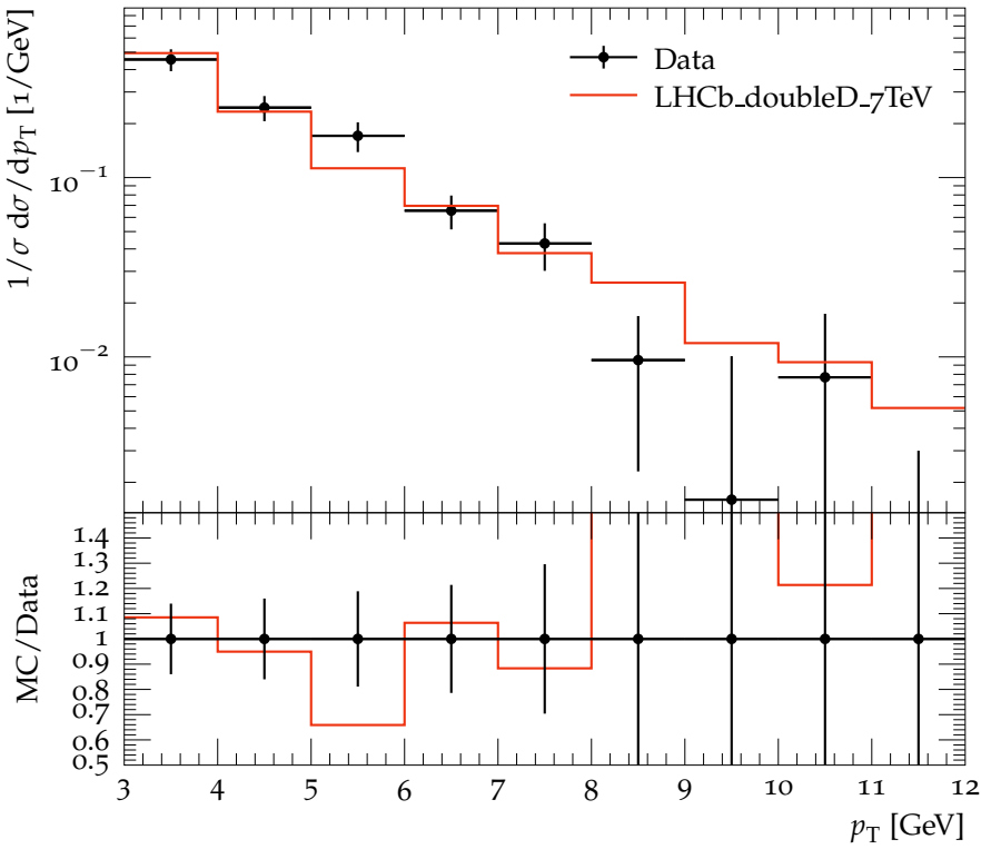
p_T distribution of D_s^+ for J/\Psi D_s^+ pairs
