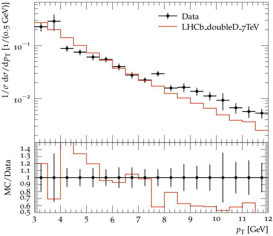
p_T distribution of charmed hadrons for D^0D^+ pairs
