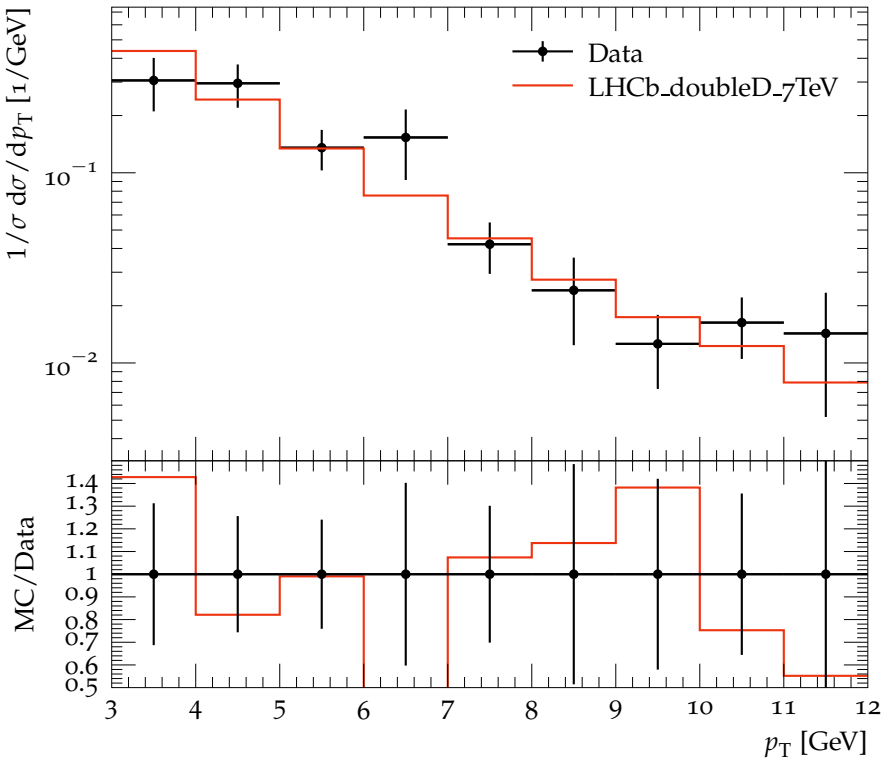
p_T distribution of D mesons for D^0 D_s^+ pairs
