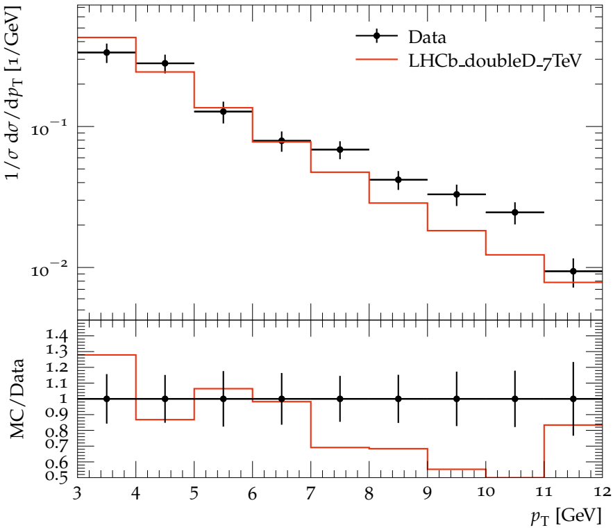
p_T distribution of charmed hadrons for D^+D_s^- pairs
