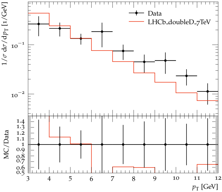
p_T distribution of charmed hadrons for D^+ \Lambda_c^- pairs
