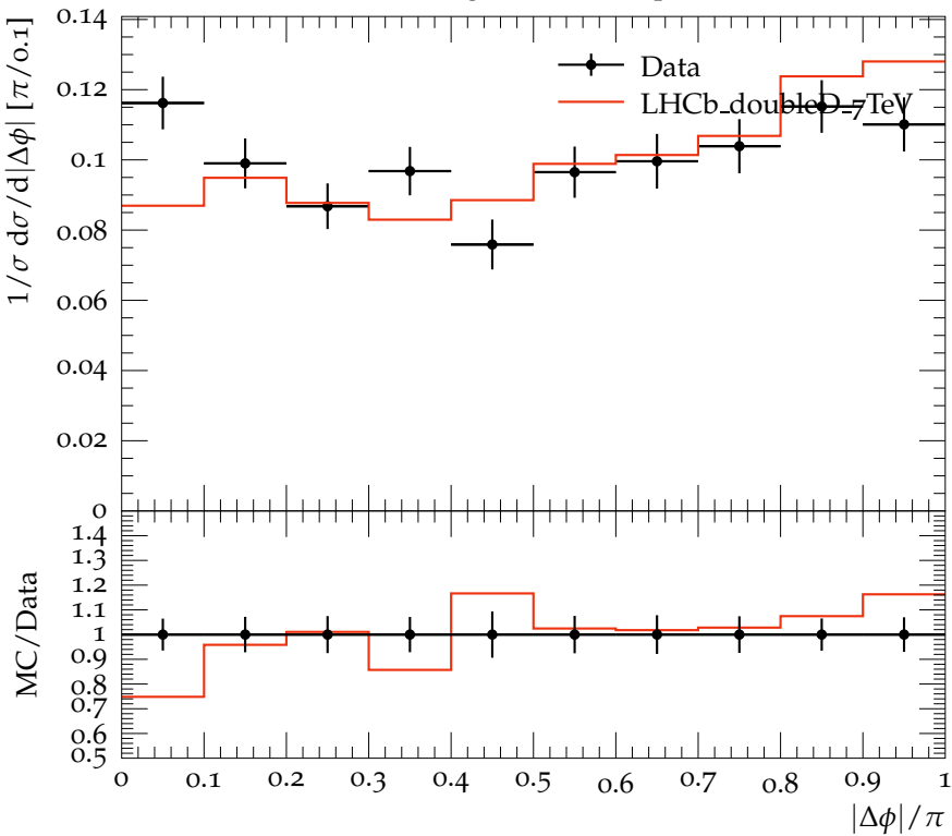
Difference in azimuthal angle for J/\Psi D^0 pairs
