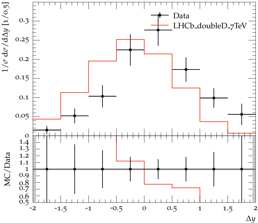
Difference in pseudorapidity for J/\Psi D_s^+ pairs
