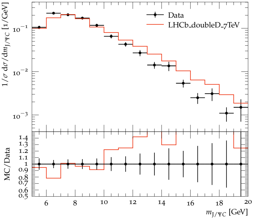
Invariant mass distribution of J/\Psi D^+ pairs
