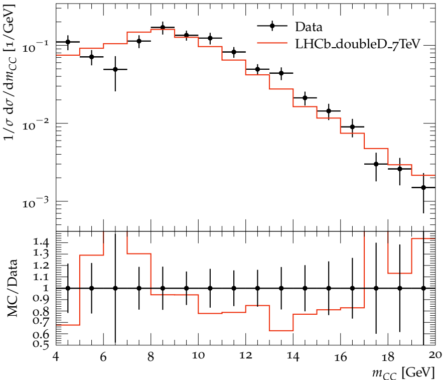
Invariant mass distribution of D^0\bar{D}^0 pairs
