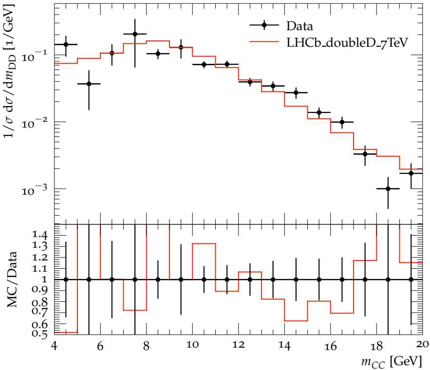
Invariant mass distribution of D^0D^+ pairs
