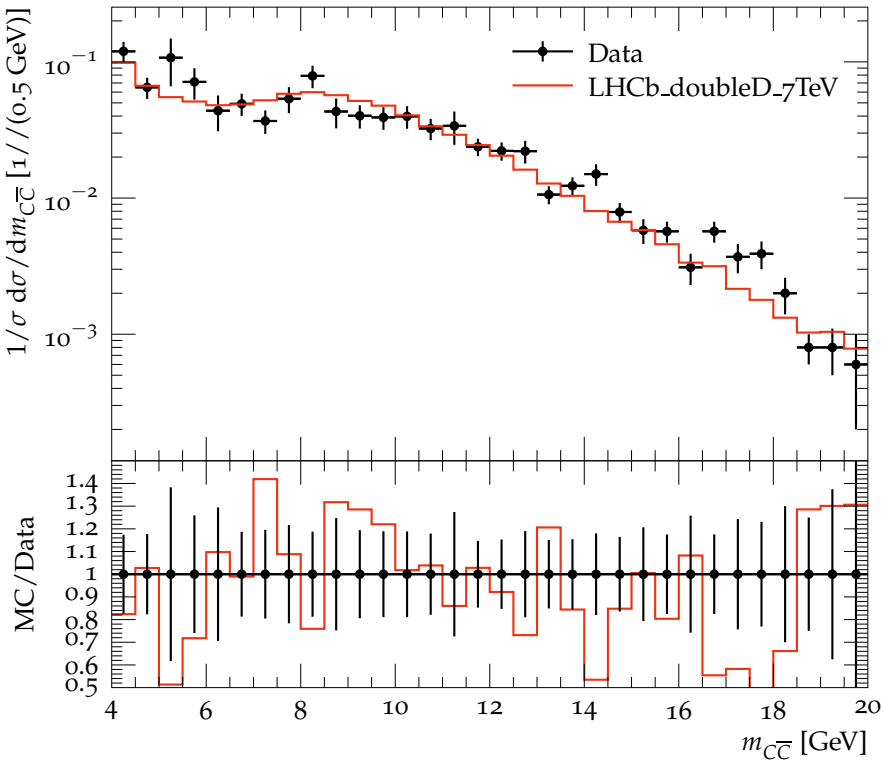
Invariant mass distribution of D^+D^- pairs
