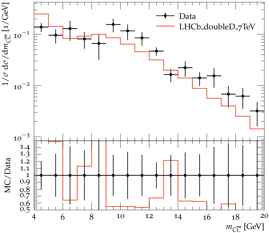
Invariant mass distribution of D^+D_s^- pairs
