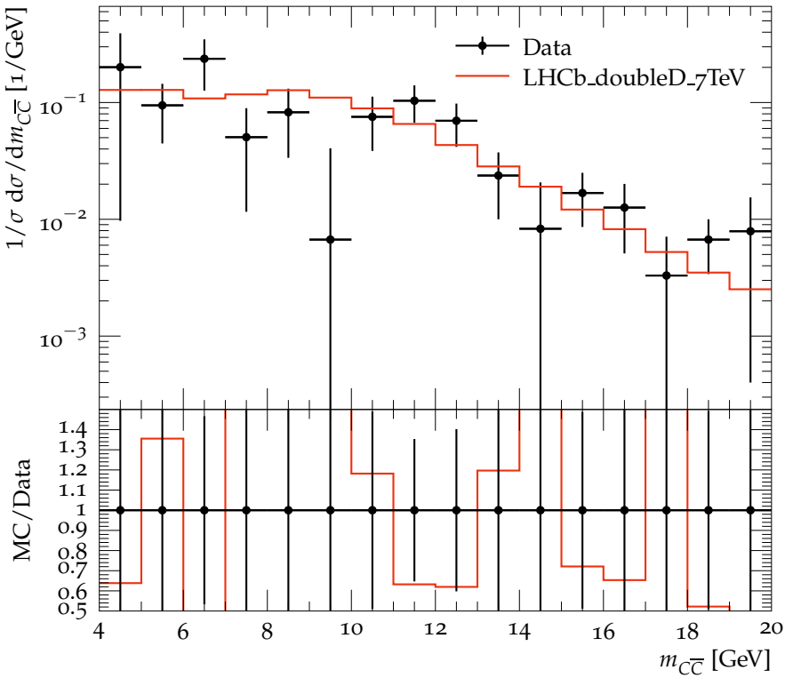
Invariant mass distribution of D^+ \Lambda_c^- pairs
