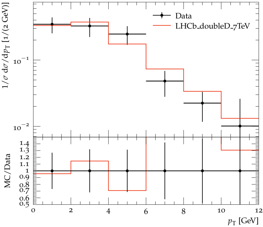
p_T distribution of J/\Psi for J/\Psi\Lambda_c^+ pairs
