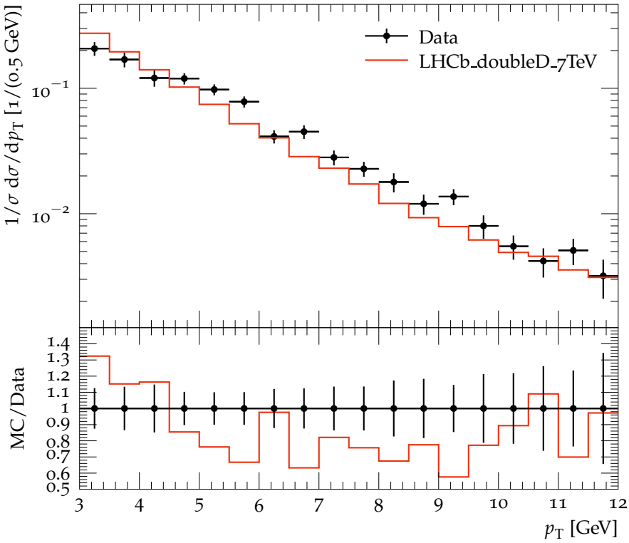
p_T distribution of charmed hadrons for D^0\bar{D}^0 pairs
