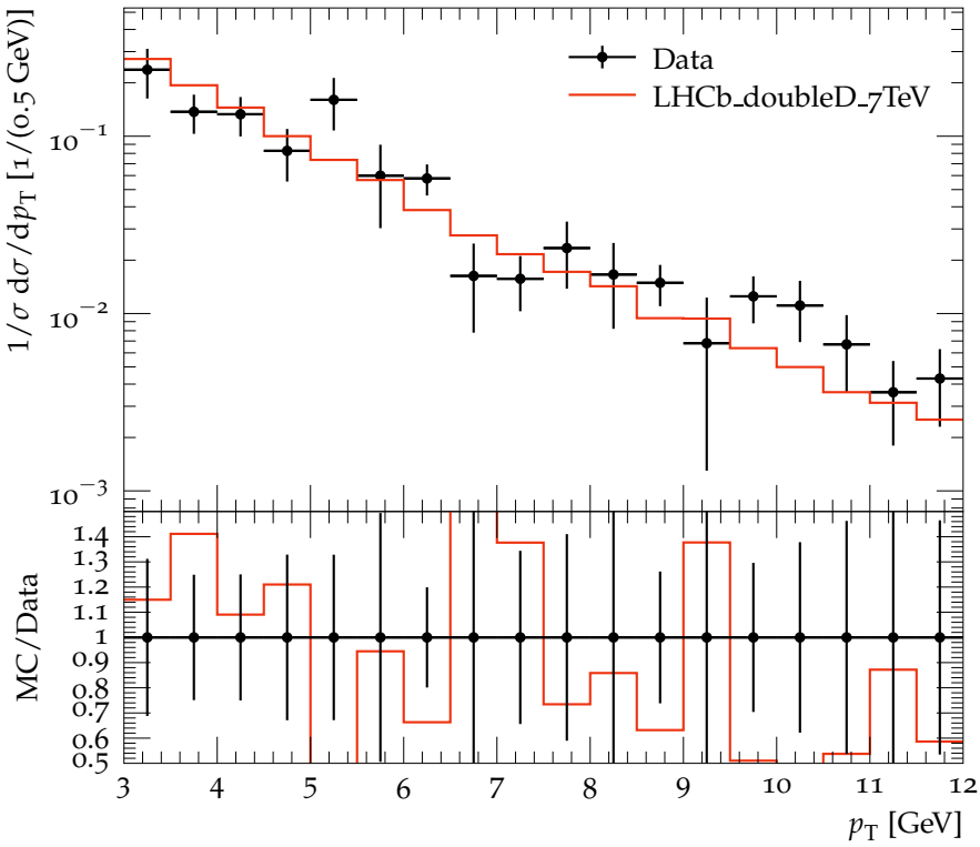
p_T distribution of charmed hadrons for D^+D^+ pairs
