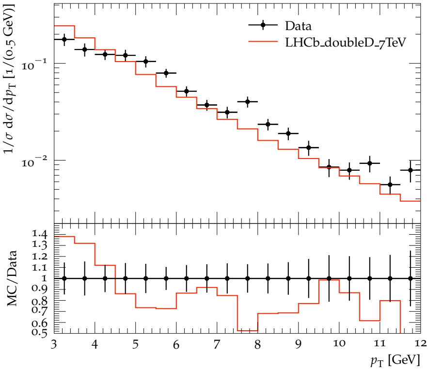
p_T distribution of charmed hadrons for D^0 D_s^- pairs
