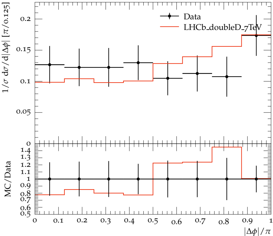
Difference in azimuthal angle for J/\Psi D_s^+ pairs
