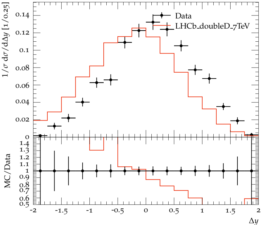
Difference in pseudorapidity for J/\Psi D^0 pairs
