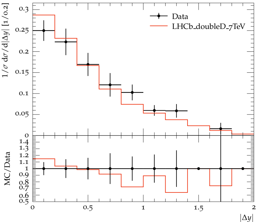
Difference in pseudorapidity for D^0D_s^- pairs
