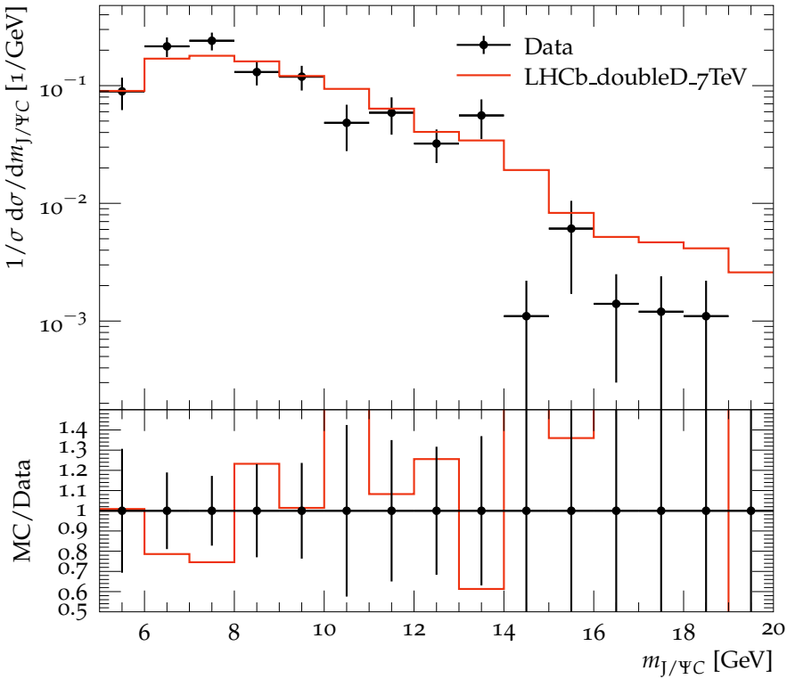
Invariant mass distribution of J/\Psi D_s^+ pairs
