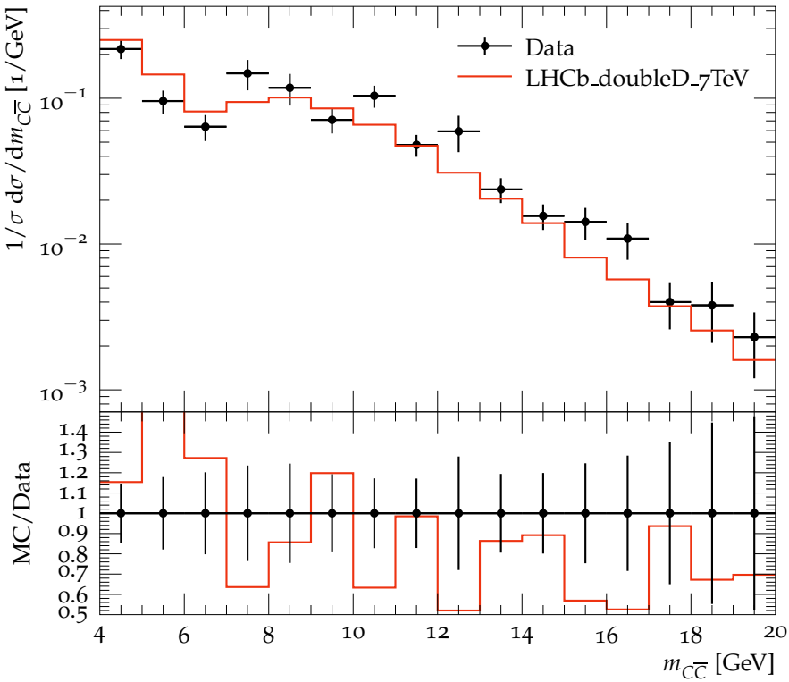
Invariant mass distribution of D^0 D_s^- pairs
