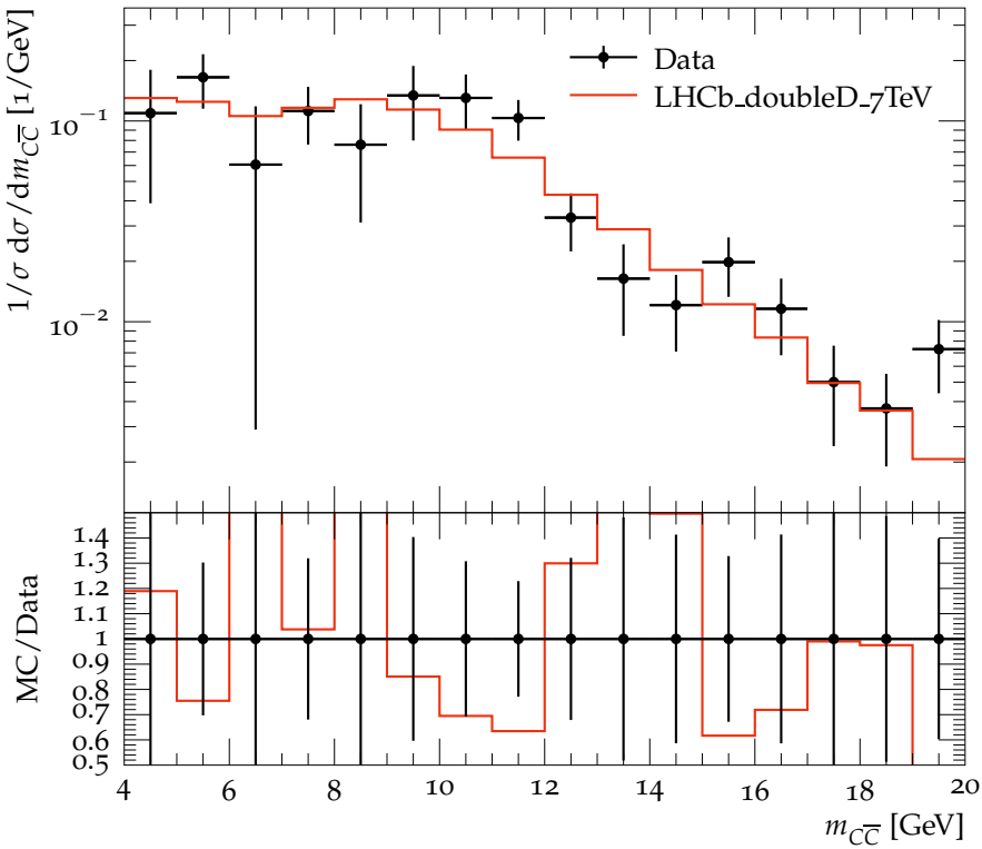
Invariant mass distribution of D^0 \Lambda_c^- pairs
